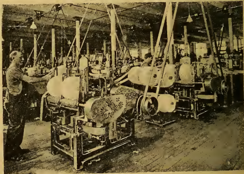
GILLING AND MAKING TOP AFTER COMBING
